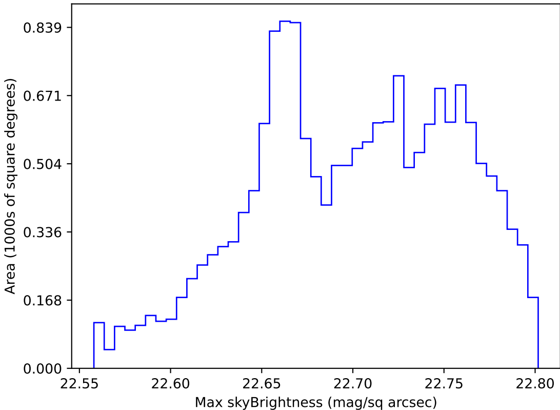
extra_ss_neo3_v3.4_10yrs WFD u band: Max skyBrightness
