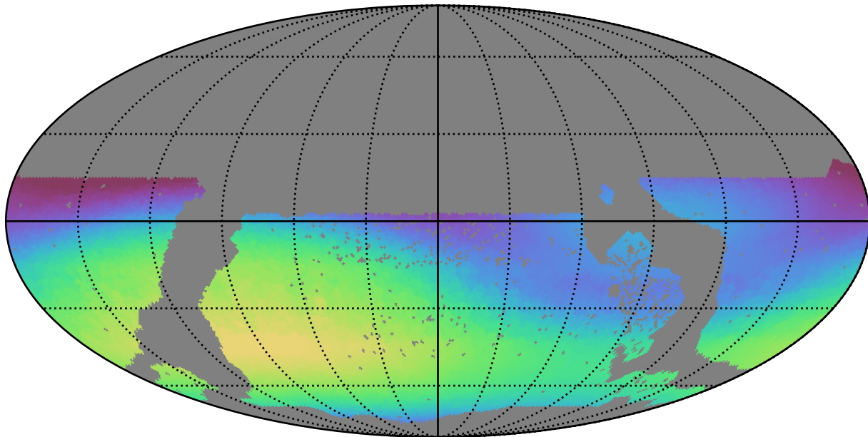
extra_ss_neo3_v3.4_10yrs WFD r band: Max skyBrightness
