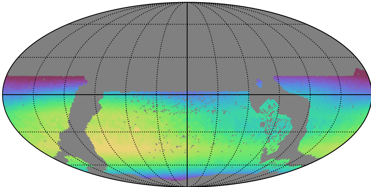
extra_ss_neo3_v3.4_10yrs WFD i band: Max skyBrightness
