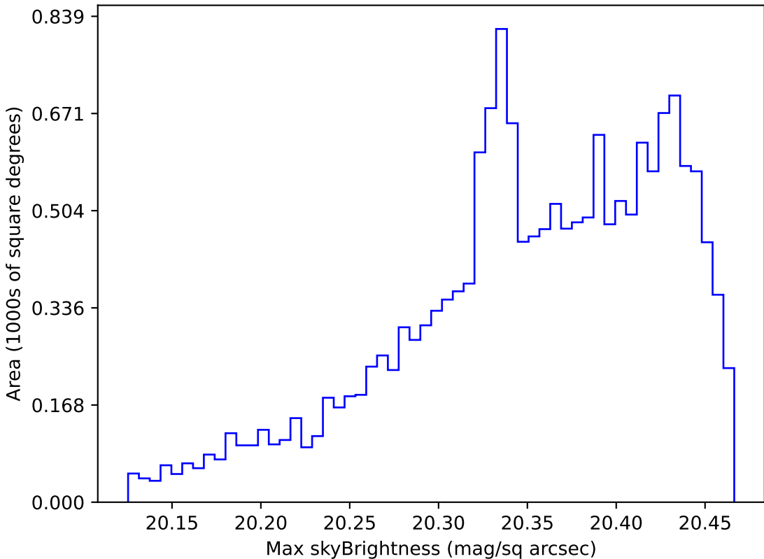
extra_ss_neo3_v3.4_10yrs WFD i band: Max skyBrightness
