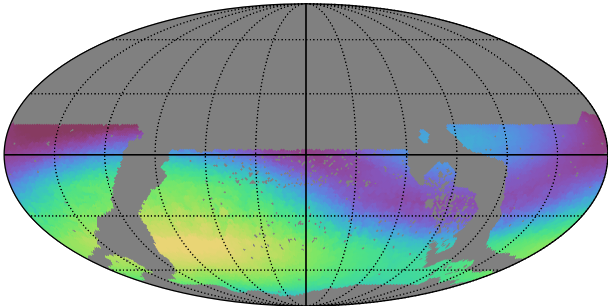
extra_ss_neo3_v3.4_10yrs WFD g band: Max skyBrightness
