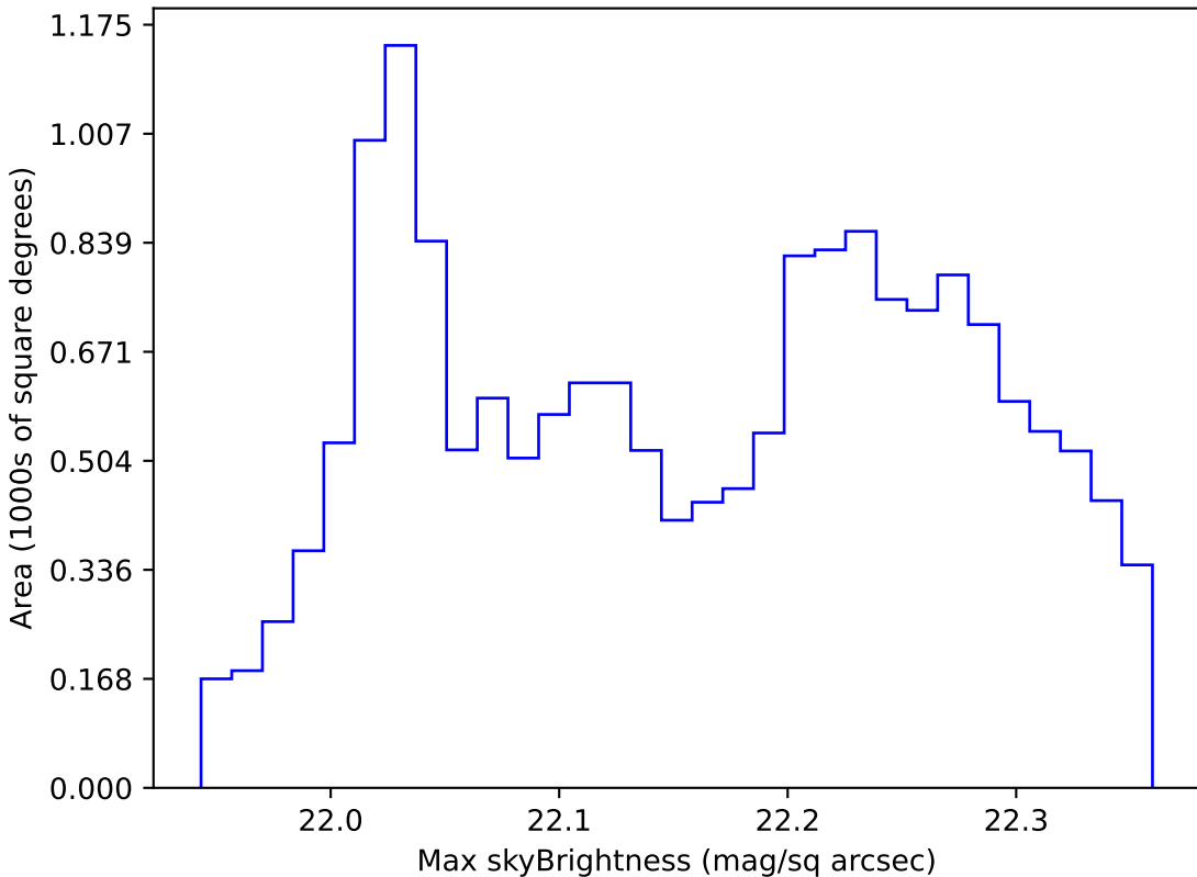
extra_ss_neo3_v3.4_10yrs WFD g band: Max skyBrightness
