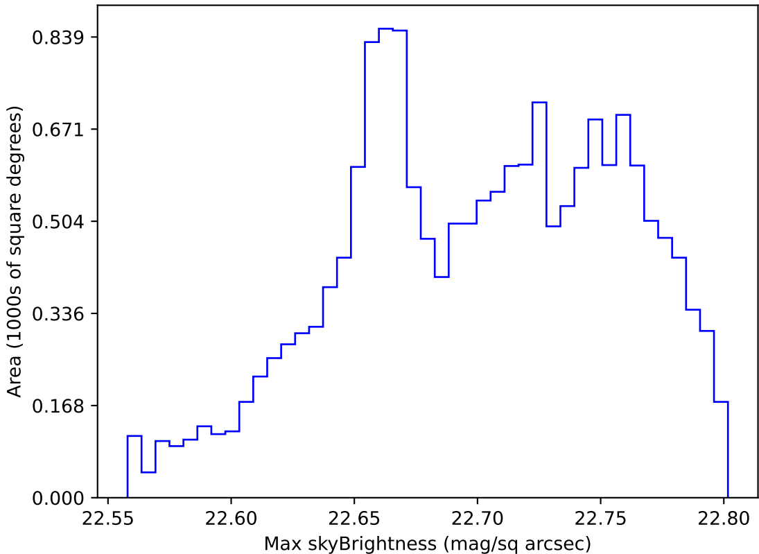
extra_ss_neo3_v3.4_10yrs WFD all bands: Max skyBrightness
