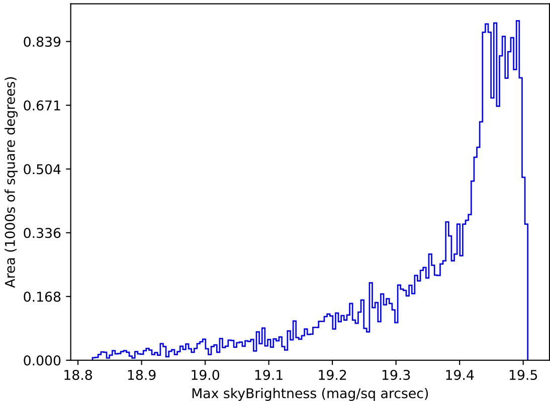
extra_ss_neo3_v3.4_10yrs All sky z band: Max skyBrightness
