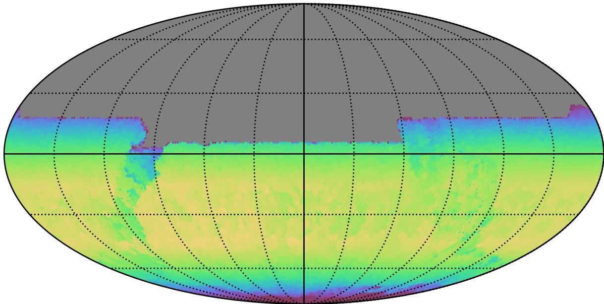
extra_ss_neo3_v3.4_10yrs All sky y band: Max skyBrightness
