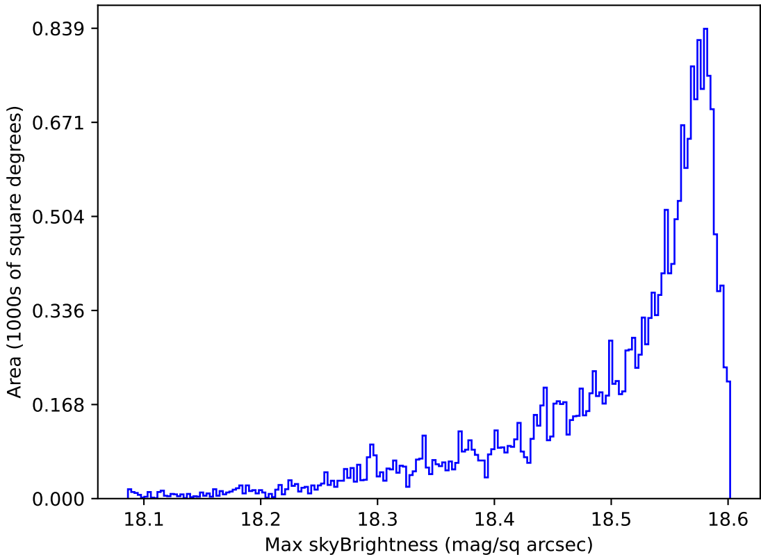
extra_ss_neo3_v3.4_10yrs All sky y band: Max skyBrightness
