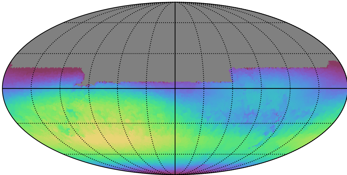
extra_ss_neo3_v3.4_10yrs All sky u band: Max skyBrightness
