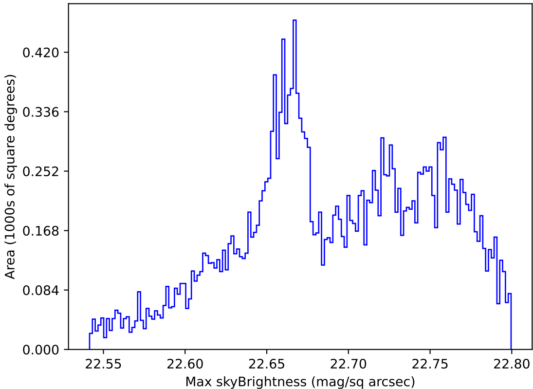
extra_ss_neo3_v3.4_10yrs All sky u band: Max skyBrightness
