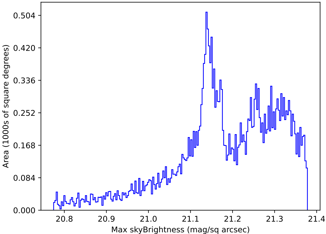
extra_ss_neo3_v3.4_10yrs All sky r band: Max skyBrightness
