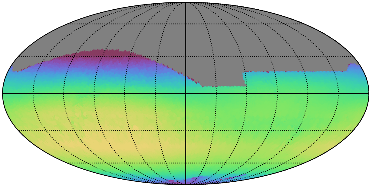
extra_ss_neo3_v3.4_10yrs All sky i band: Max skyBrightness
