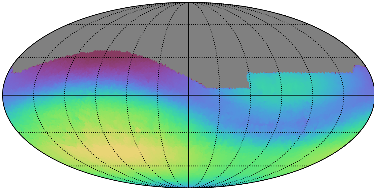
extra_ss_neo3_v3.4_10yrs All sky g band: Max skyBrightness
