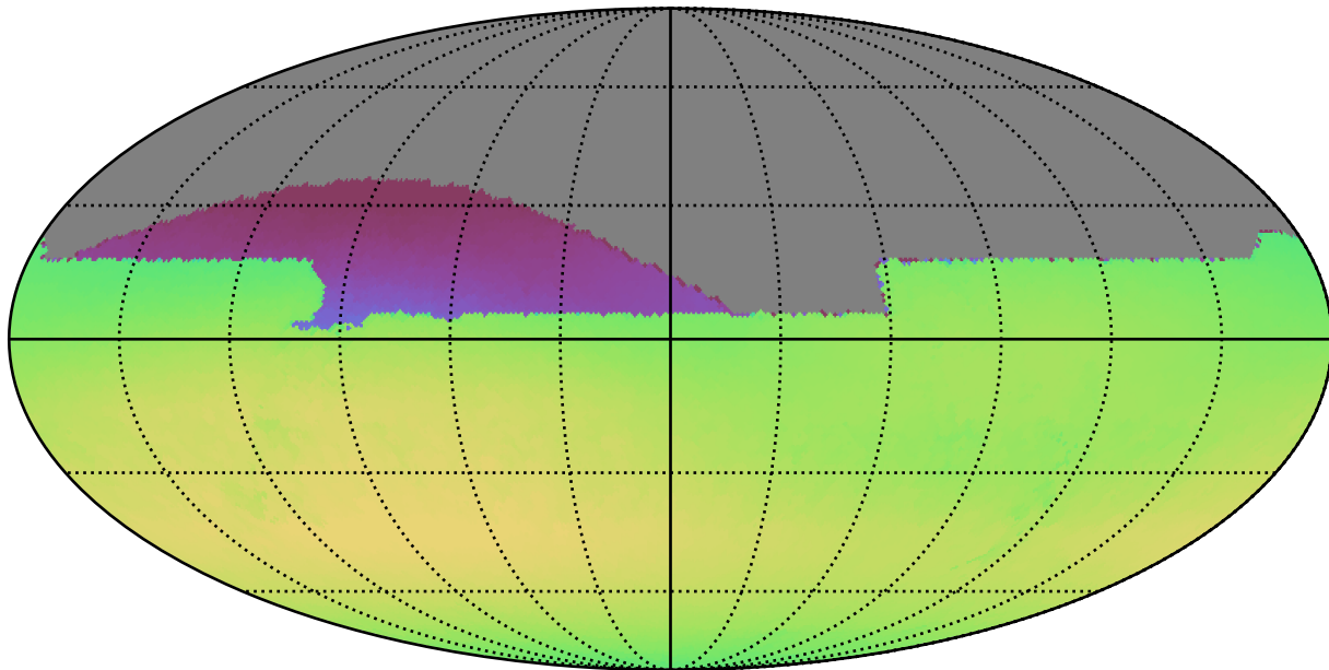
extra_ss_neo3_v3.4_10yrs All sky all bands: Max skyBrightness
