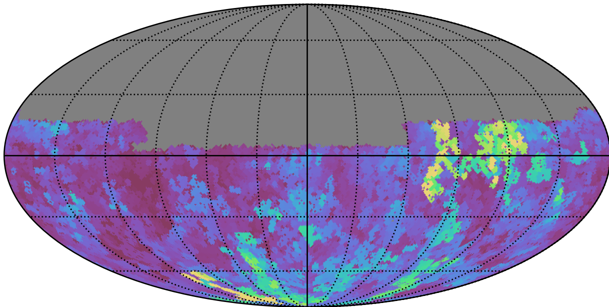
extra_ss_neo3_v3.4_10yrs Yr 1 u band: Max seeingGeom
