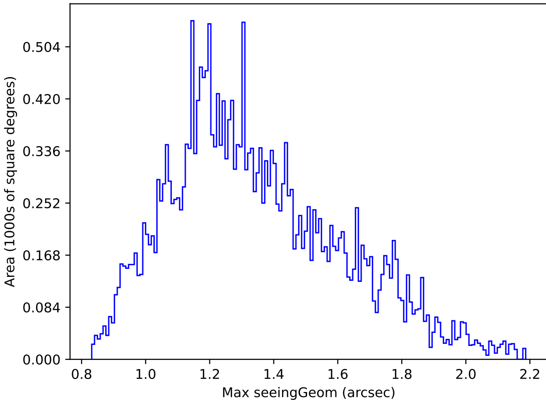
extra_ss_neo3_v3.4_10yrs Yr 1 r band: Max seeingGeom
