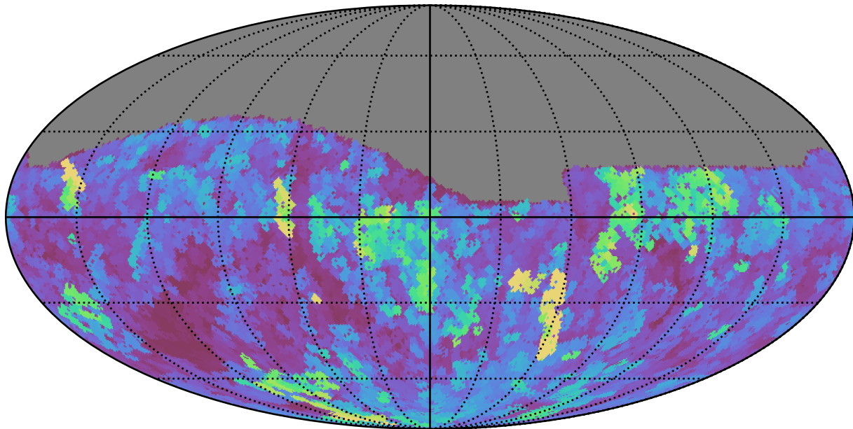
extra_ss_neo3_v3.4_10yrs Yr 1 all bands: Max seeingGeom
