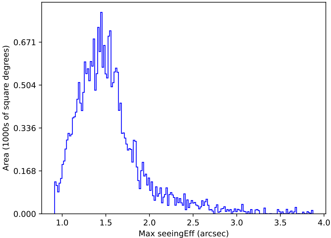
extra_ss_neo3_v3.4_10yrs Yr 1 z band: Max seeingEff
