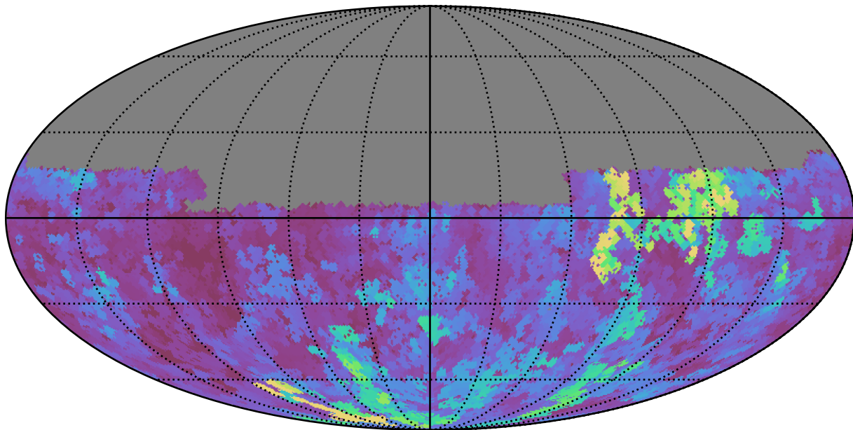
extra_ss_neo3_v3.4_10yrs Yr 1 u band: Max seeingEff
