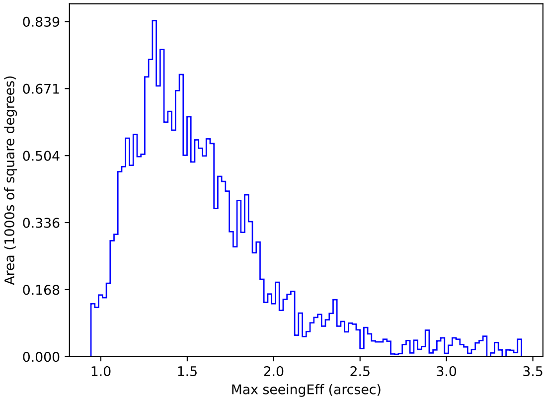
extra_ss_neo3_v3.4_10yrs Yr 1 u band: Max seeingEff
