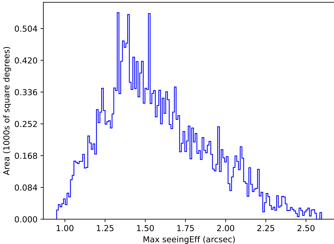
extra_ss_neo3_v3.4_10yrs Yr 1 r band: Max seeingEff
