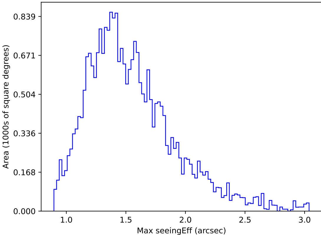
extra_ss_neo3_v3.4_10yrs Yr 1 i band: Max seeingEff
