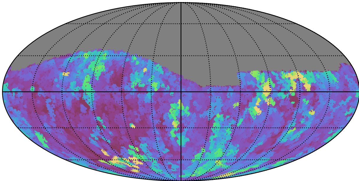
extra_ss_neo3_v3.4_10yrs Yr 1 g band: Max seeingEff
