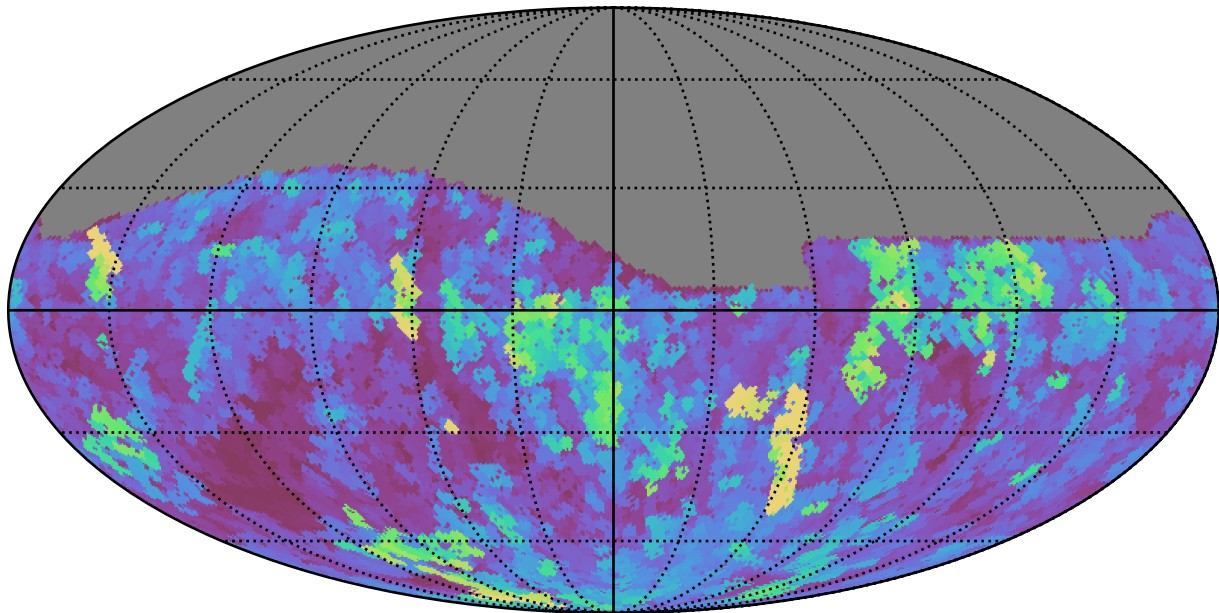
extra_ss_neo3_v3.4_10yrs Yr 1 all bands: Max seeingEff
