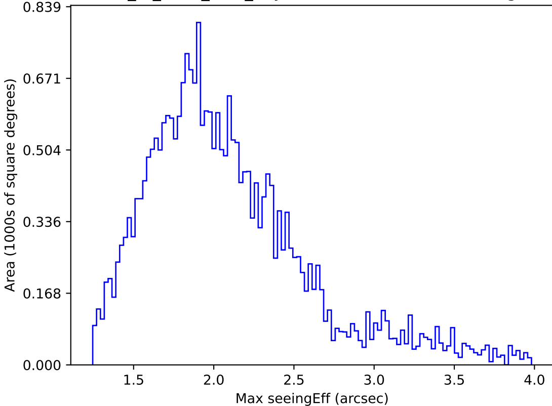
extra_ss_neo3_v3.4_10yrs Yr 1 all bands: Max seeingEff
