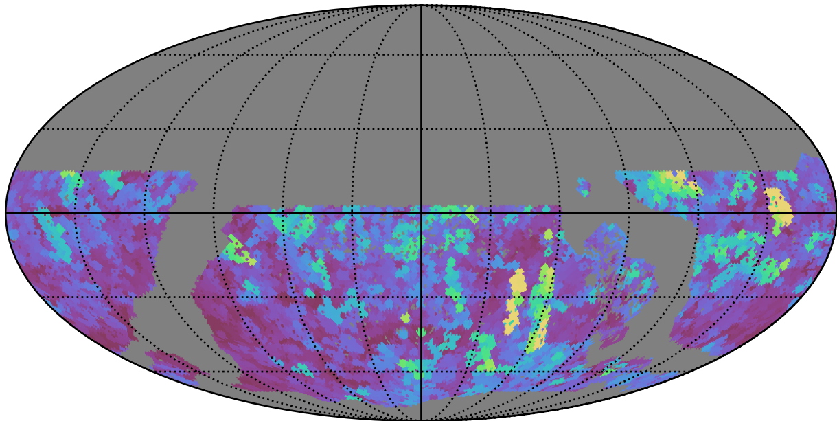
extra_ss_neo3_v3.4_10yrs WFD z band: Max seeingEff
