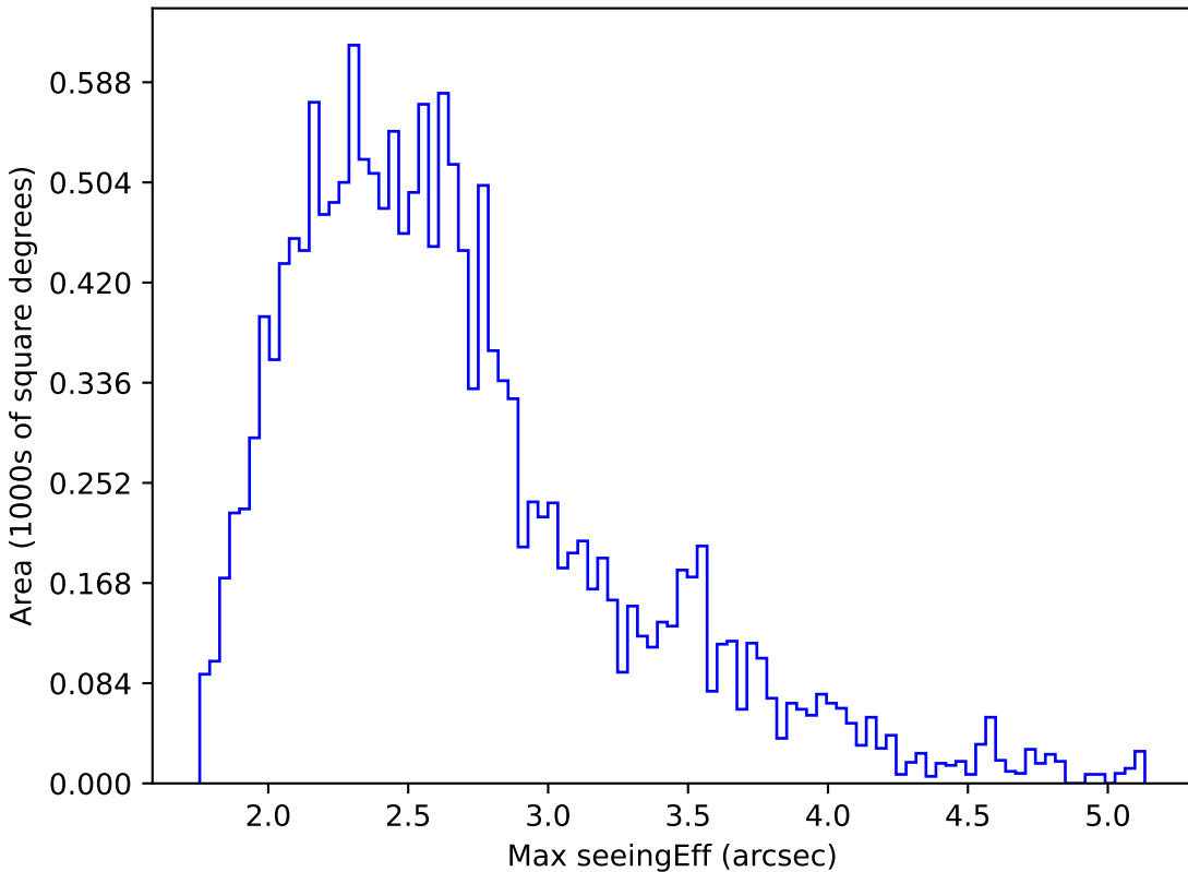
extra_ss_neo3_v3.4_10yrs WFD z band: Max seeingEff
