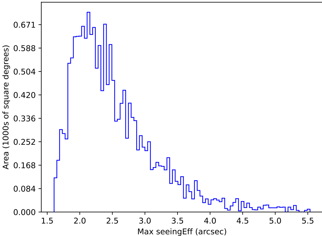
extra_ss_neo3_v3.4_10yrs WFD y band: Max seeingEff
