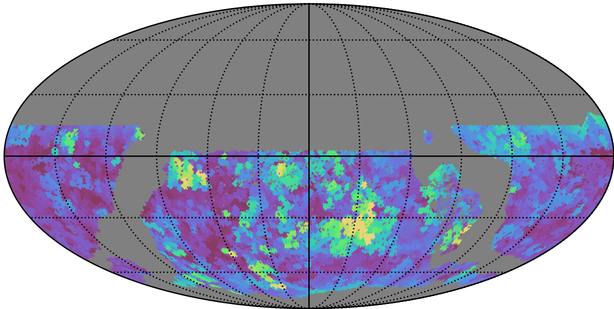
extra_ss_neo3_v3.4_10yrs WFD u band: Max seeingEff
