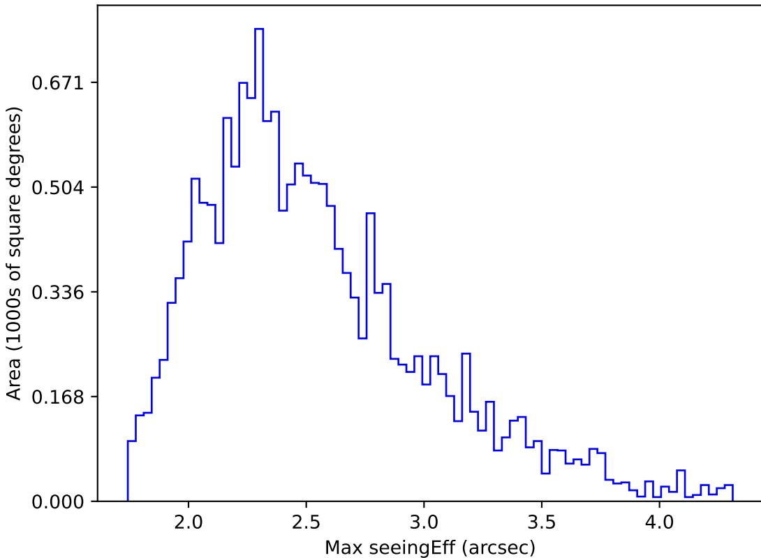
extra_ss_neo3_v3.4_10yrs WFD u band: Max seeingEff
