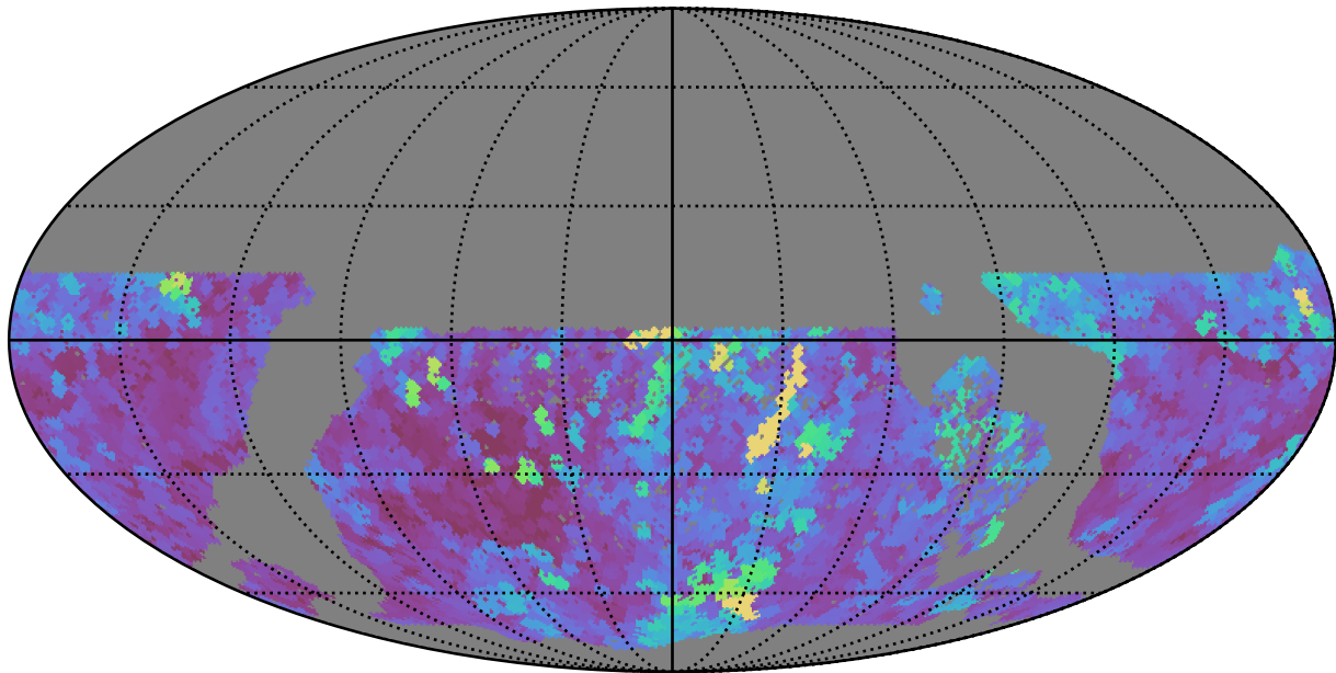
extra_ss_neo3_v3.4_10yrs WFD r band: Max seeingEff
