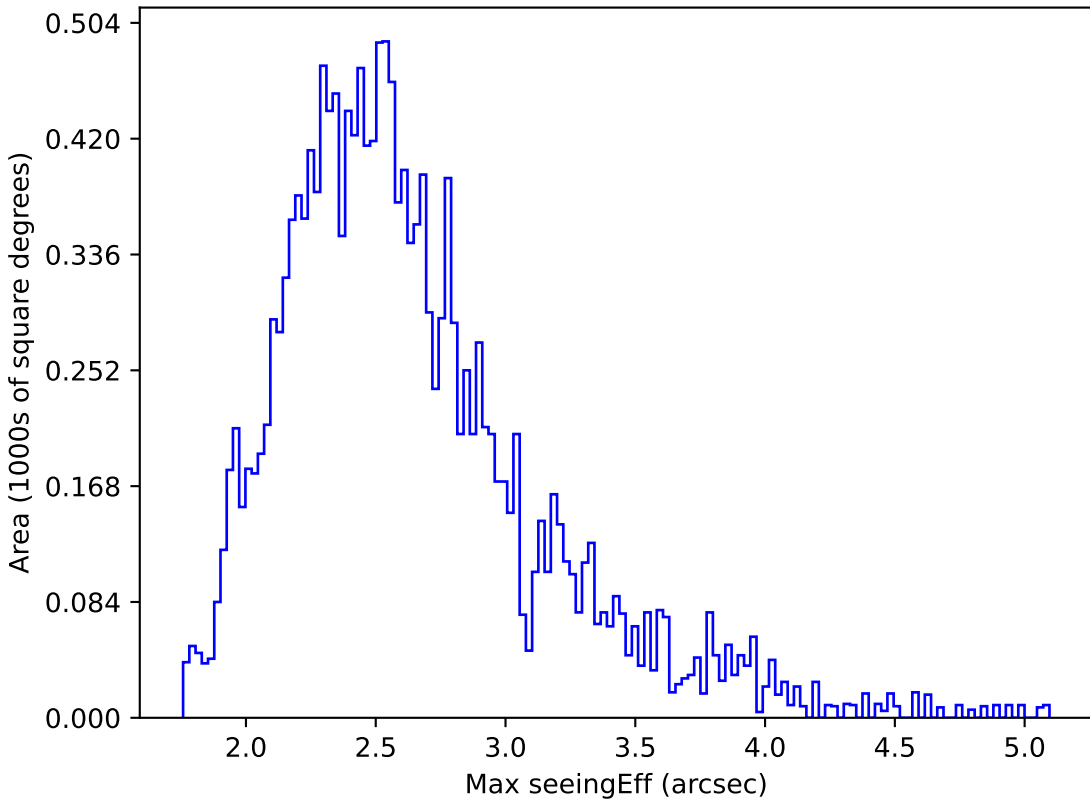
extra_ss_neo3_v3.4_10yrs WFD r band: Max seeingEff
