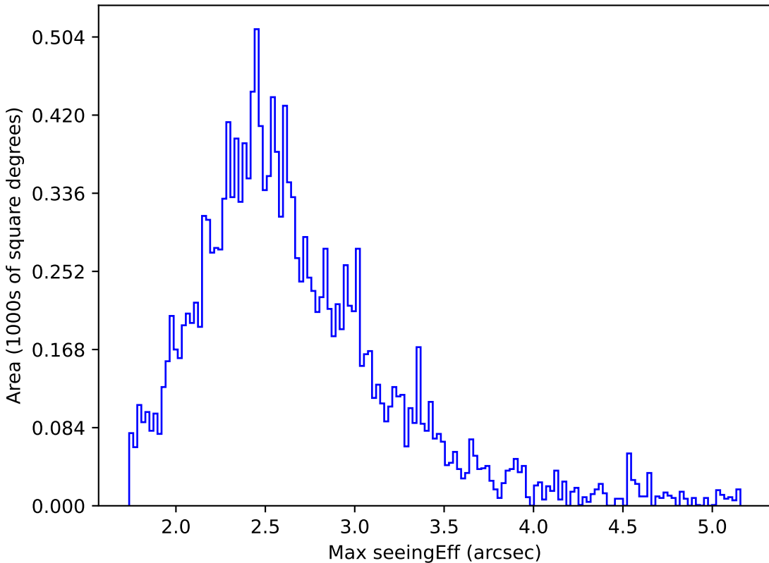
extra_ss_neo3_v3.4_10yrs WFD i band: Max seeingEff
