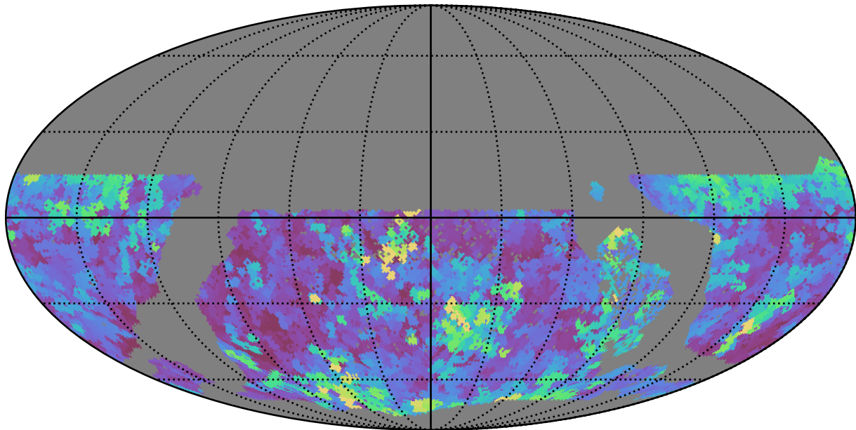
extra_ss_neo3_v3.4_10yrs WFD g band: Max seeingEff
