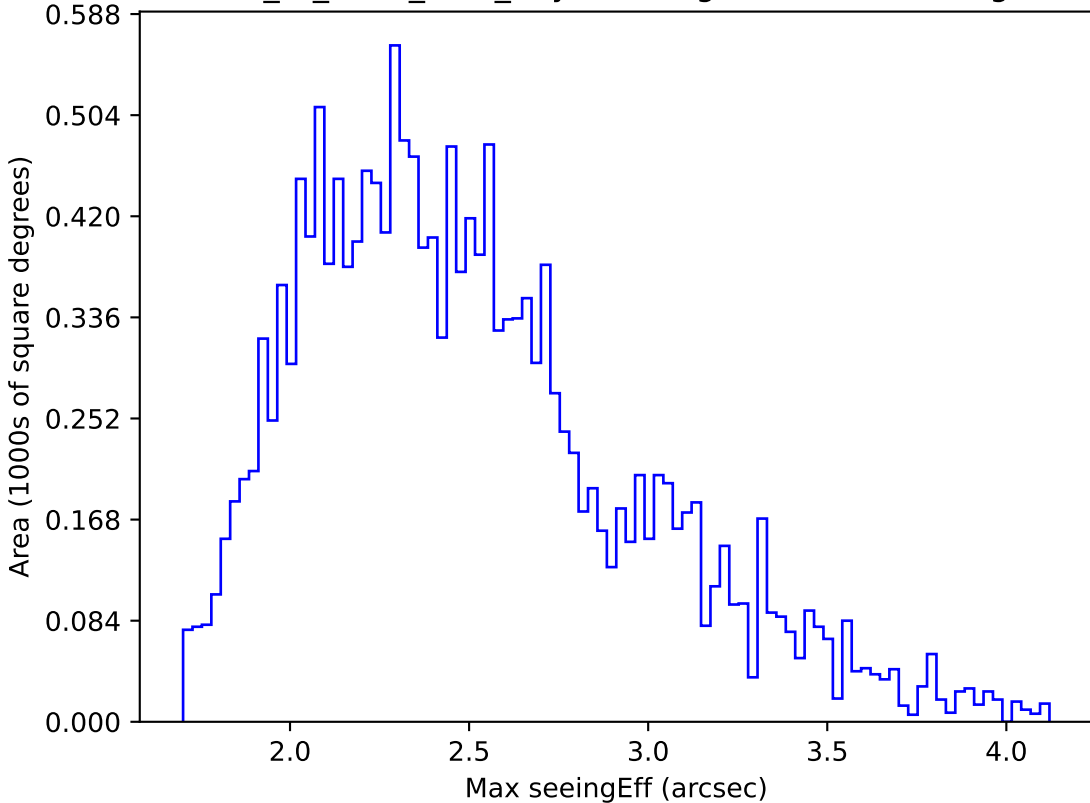
extra_ss_neo3_v3.4_10yrs WFD g band: Max seeingEff
