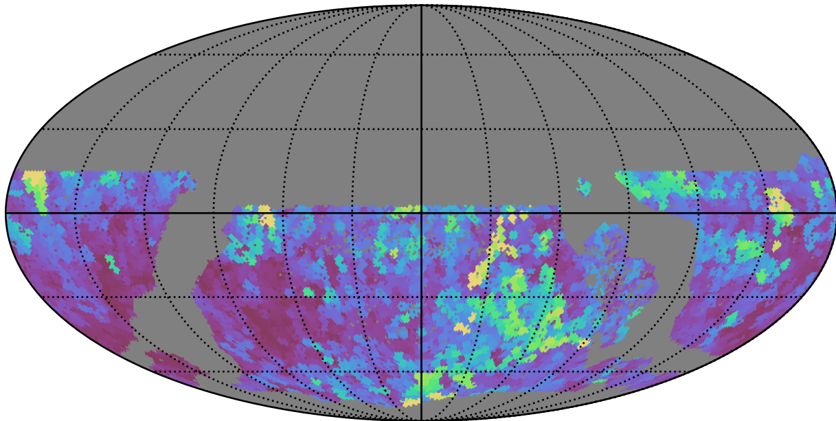
extra_ss_neo3_v3.4_10yrs WFD all bands: Max seeingEff
