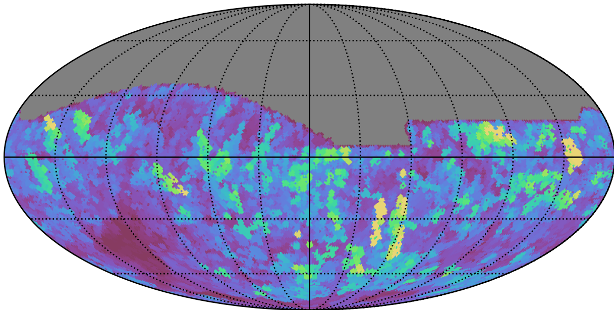
extra_ss_neo3_v3.4_10yrs All sky z band: Max seeingEff
