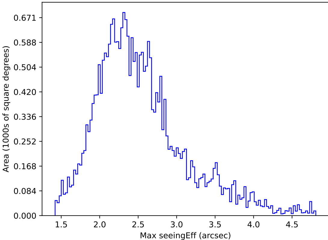
extra_ss_neo3_v3.4_10yrs All sky z band: Max seeingEff
