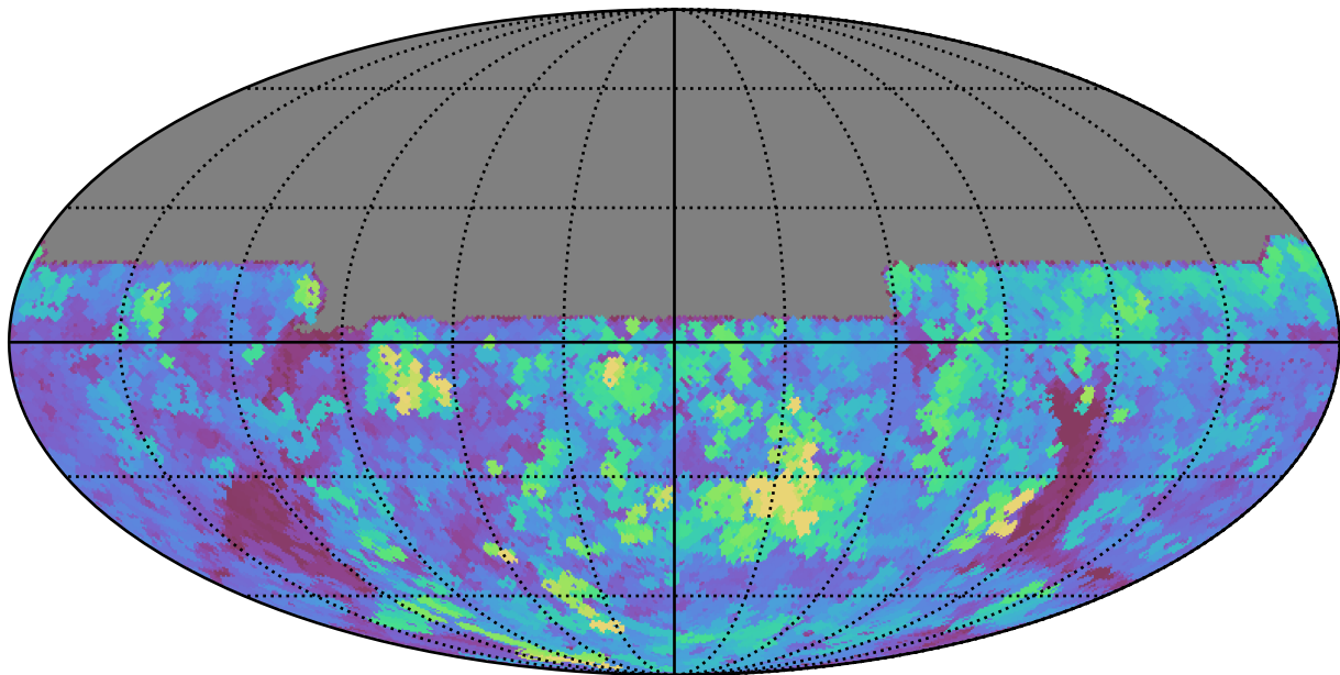
extra_ss_neo3_v3.4_10yrs All sky u band: Max seeingEff
