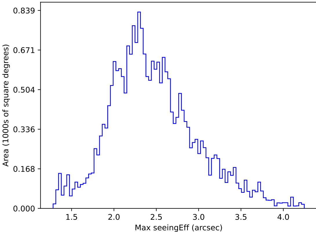
extra_ss_neo3_v3.4_10yrs All sky u band: Max seeingEff
