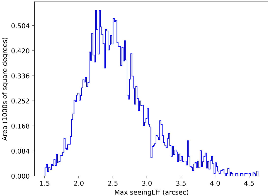
extra_ss_neo3_v3.4_10yrs All sky r band: Max seeingEff
