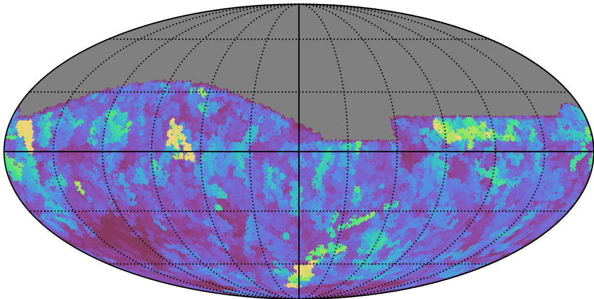
extra_ss_neo3_v3.4_10yrs All sky i band: Max seeingEff
