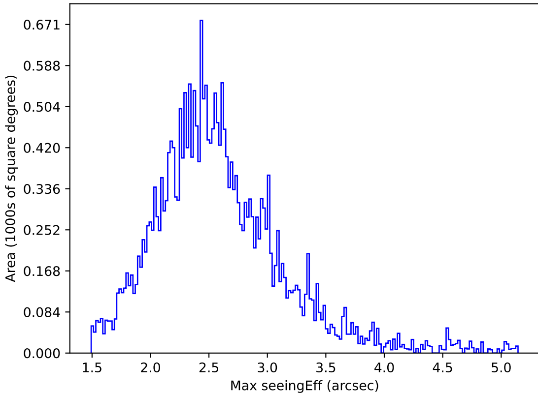
extra_ss_neo3_v3.4_10yrs All sky i band: Max seeingEff
