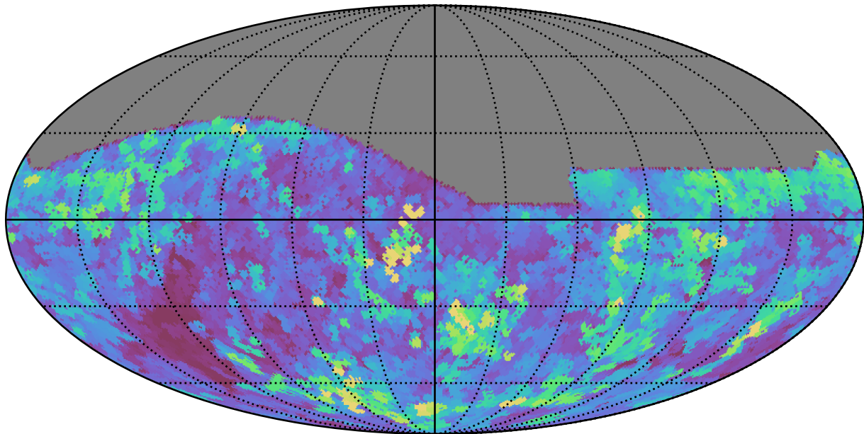
extra_ss_neo3_v3.4_10yrs All sky g band: Max seeingEff
