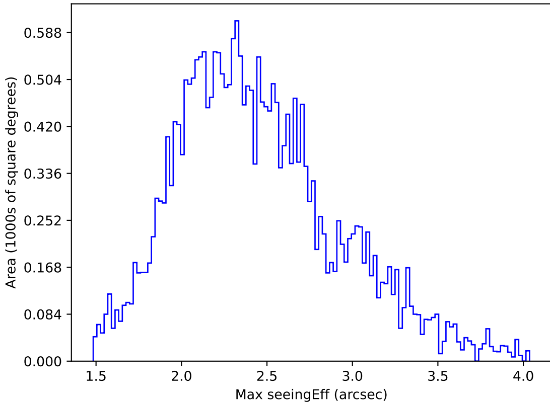
extra_ss_neo3_v3.4_10yrs All sky g band: Max seeingEff
