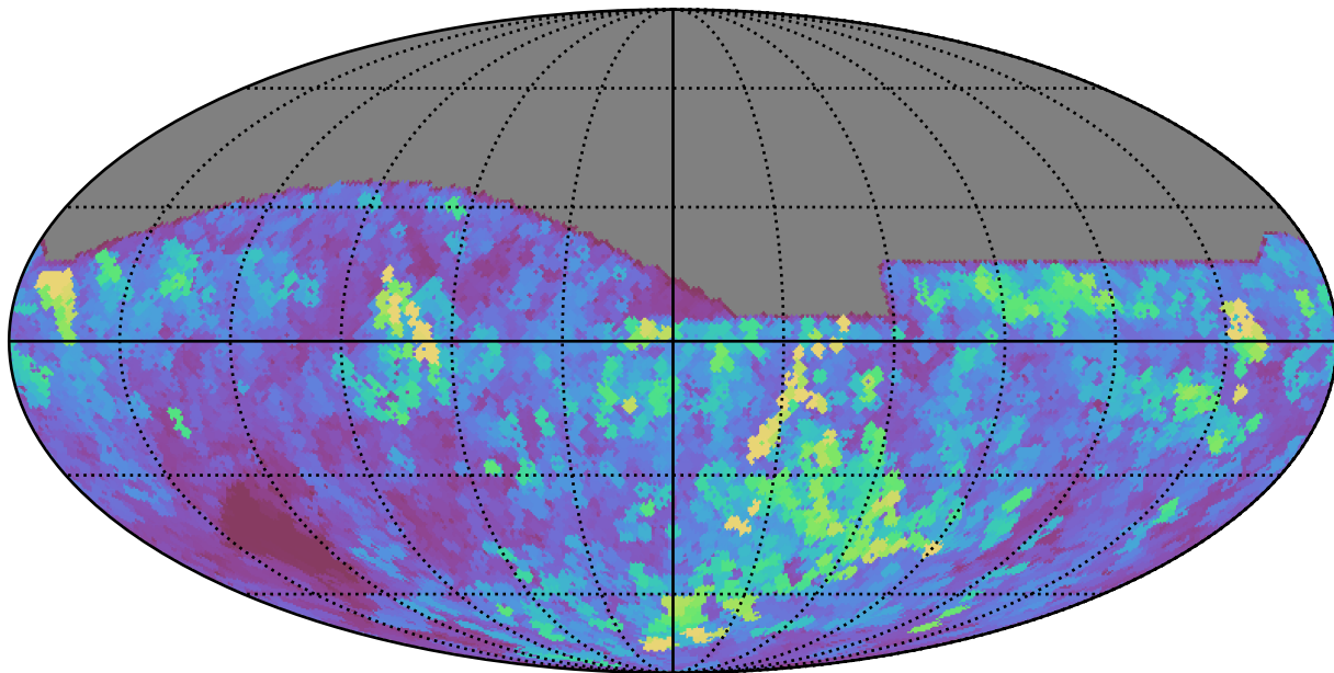
extra_ss_neo3_v3.4_10yrs All sky all bands: Max seeingEff
