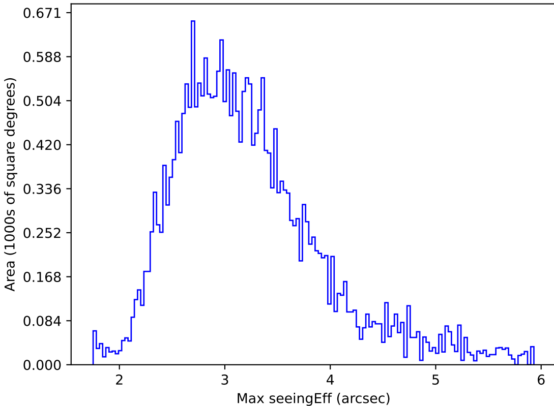
extra_ss_neo3_v3.4_10yrs All sky all bands: Max seeingEff
