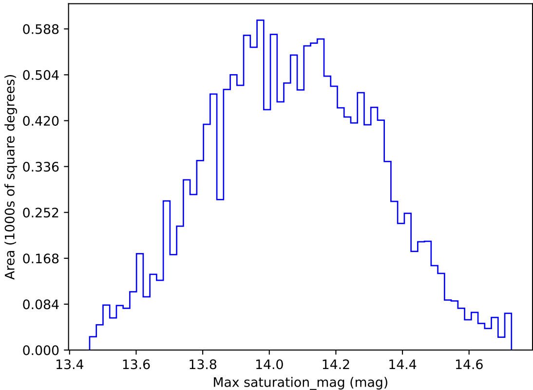
extra_ss_neo3_v3.4_10yrs WFD u band: Max saturation_mag
